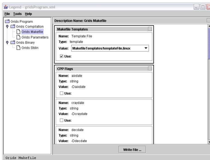
Figure 4-3: Example of a set of opened LCML description files.
